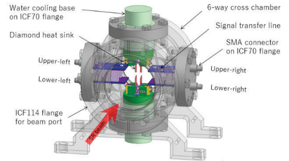
Figure 2: 3D image of the prototype.
