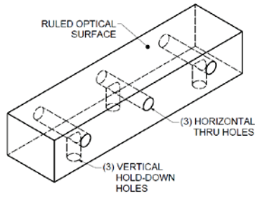
Figure 1: Grating Substrate Mounting Details.
