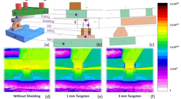
Figure 2: FLUKA simulations: (a) original CAD model; (b) upstream view of the model in FLUKA; (c) side view of the model in FLUKA; (d) to (f) upstream view of photon track length density (Particles/cm 2 /s) for three shielding designs.
