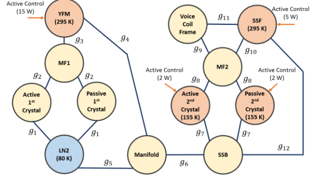
Figure 3 – Thermal Model.
