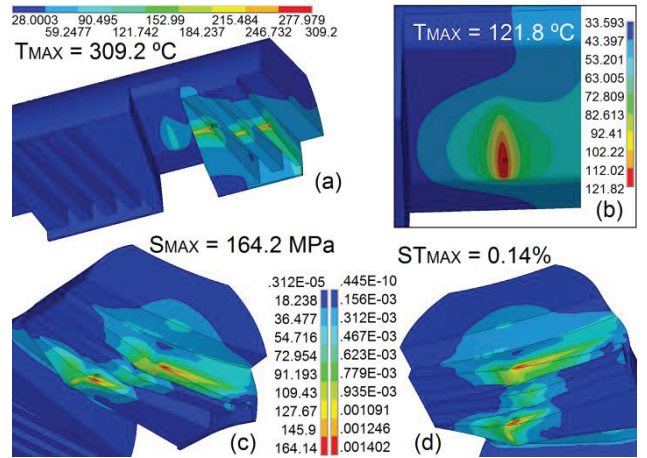
Figure 6: FEA results for the new Glidcop Al-15 crotch absorber in the dipole chamber: (a) Temperature map, (b) Local detail of the temperature distribution at the ID power deposition, (c) Stress map, and (d) Strain map.
