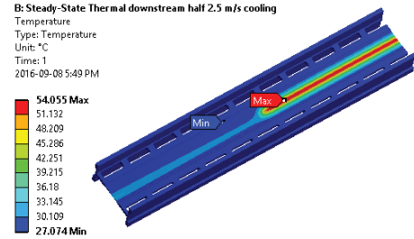
Figure 10: Downstream half chamber temperature.
