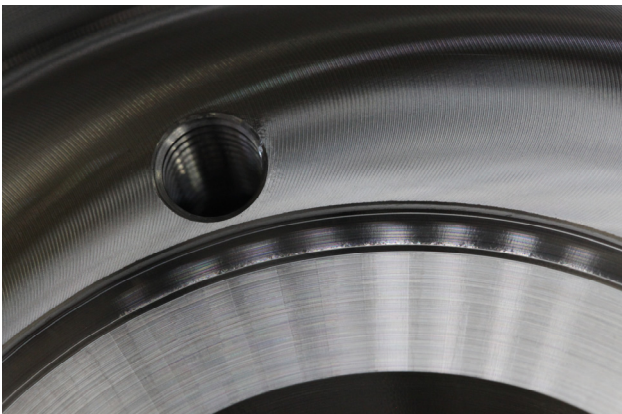
Figure 18: Last picture documents the orange skin micro damages on the scintillation screen monitor vacuum chambers for E-XFEL project.
