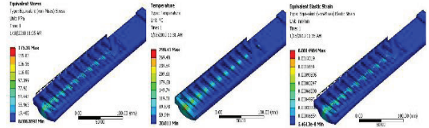
Figure 2: FEA results for absorber 2.
