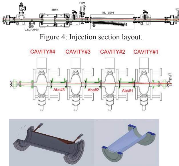
Figure 5: RF section layout, transition centre absorber and the upstream transition parts.
