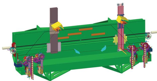
Figure 3: The optical bench as support structure for the precision mechanics and further components.
