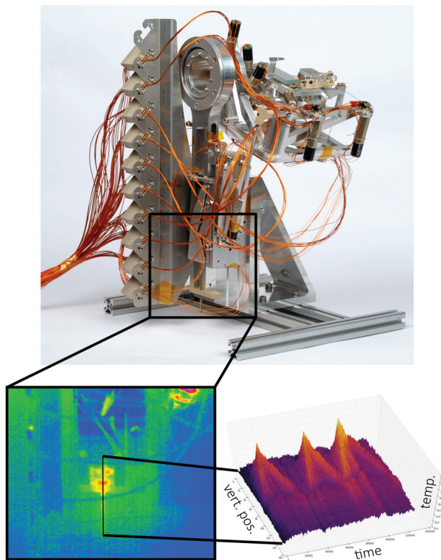
Figure 6: Photograph of the assembled and wired prototype and the results of the thermal investigation.
