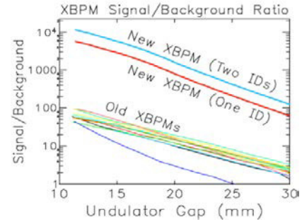
Figure 2: Ratio of undulator signal over BM background for the GRID-XBPM [2].
