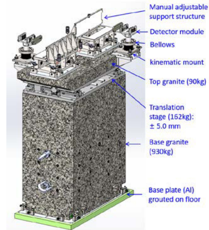
Figure 7: Support Structures.
