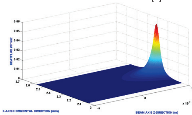
Figure 5: CSX EPU Heat Load for 0.2 mrad beam mis-steer.
