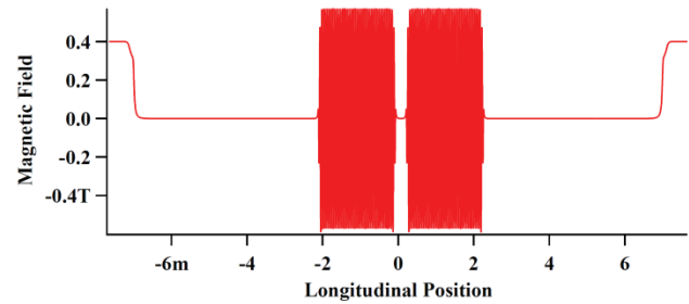
Figure 3: Magnetic Structure of CSX EPU.
