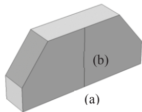
Figure 1: a cutaway view of the existing I20 monochromator crystal design. Point (a) is held fixed while line (b) is restrained in the x- and y-directions.
