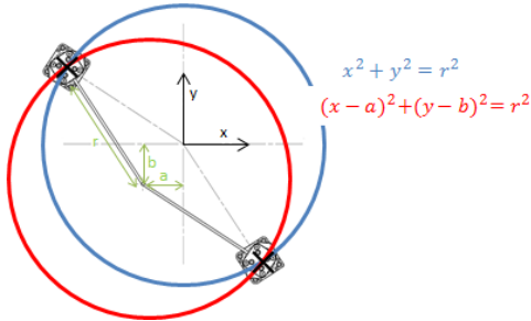
Figure 4: Polynomial equations.
