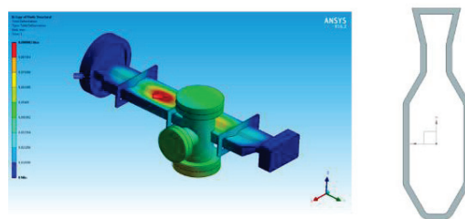
Figure 6: Straight chamber calculations and cross section
