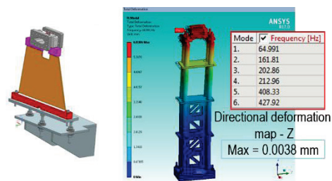
Figure 5: Downstream BPM bracket and upstream BPM support static and vibrational analysis.
