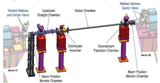
Figure 2: General assembly of stripline section.
