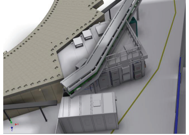
Figure 2: Optical hutch prototype – implantation to be installed in the UVX storage ring.
