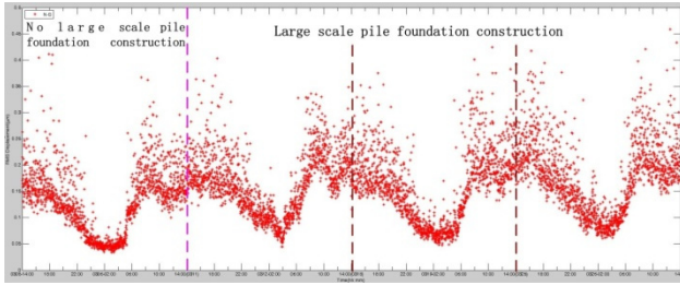
Figure 5: RMS displacements of the point A at SSRF Experimental Hall in north-south direction every Friday in March, 2015.
