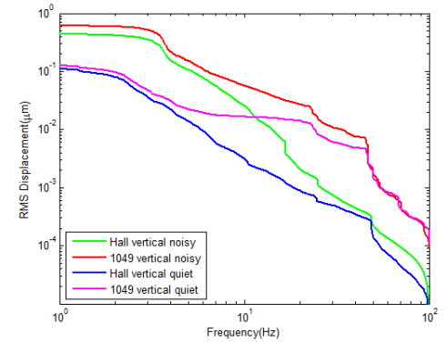
Figure 14: RMS curves of ground vibration of Point A (Hall) and Point C(Room 1049) in noisy and quiet time at SSRF in vertical direction.
