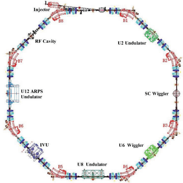
Figure 1: Layout of HLS-II storage ring.
