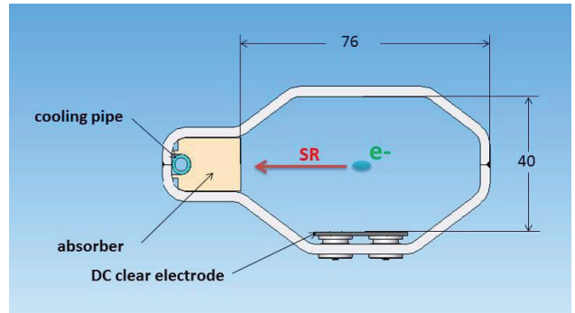
Figure 2: The section of the main vacuum pipe.
