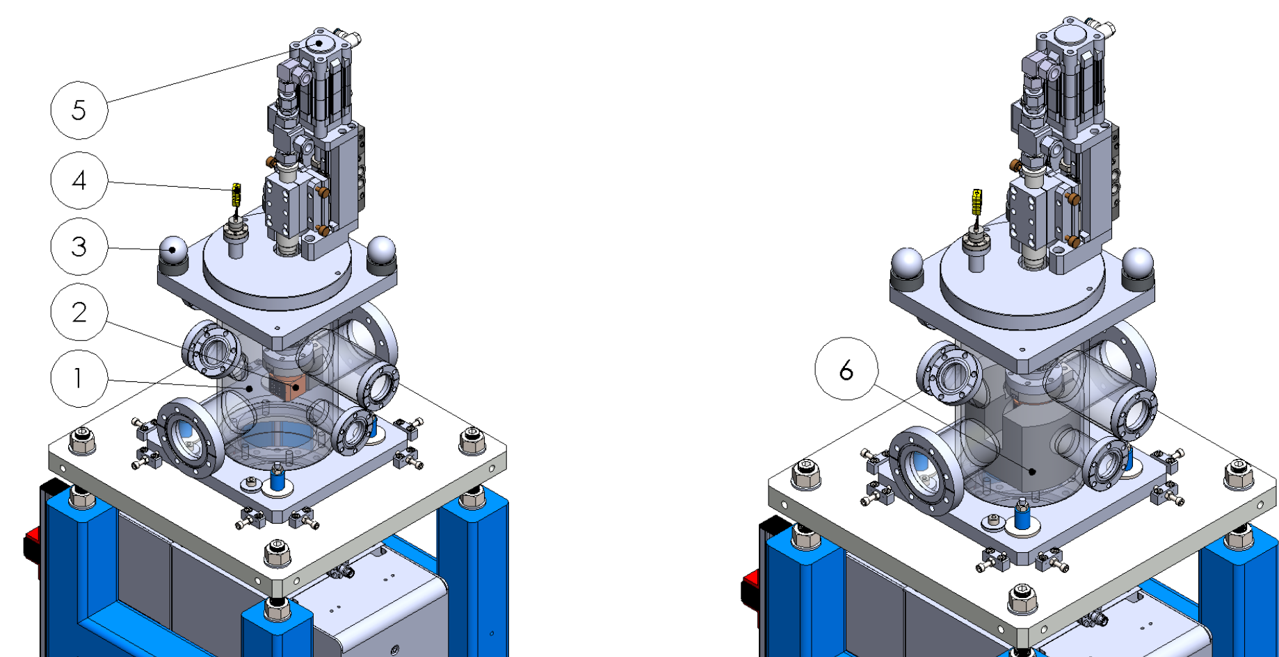
Fig. 5 The schematic drawing of the PAB.
