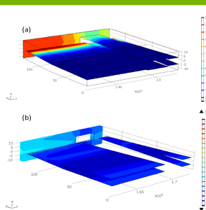
Figure 4: Temperature profile of X-ray intercepting surface (a) All-Cu body design (b) VA design
