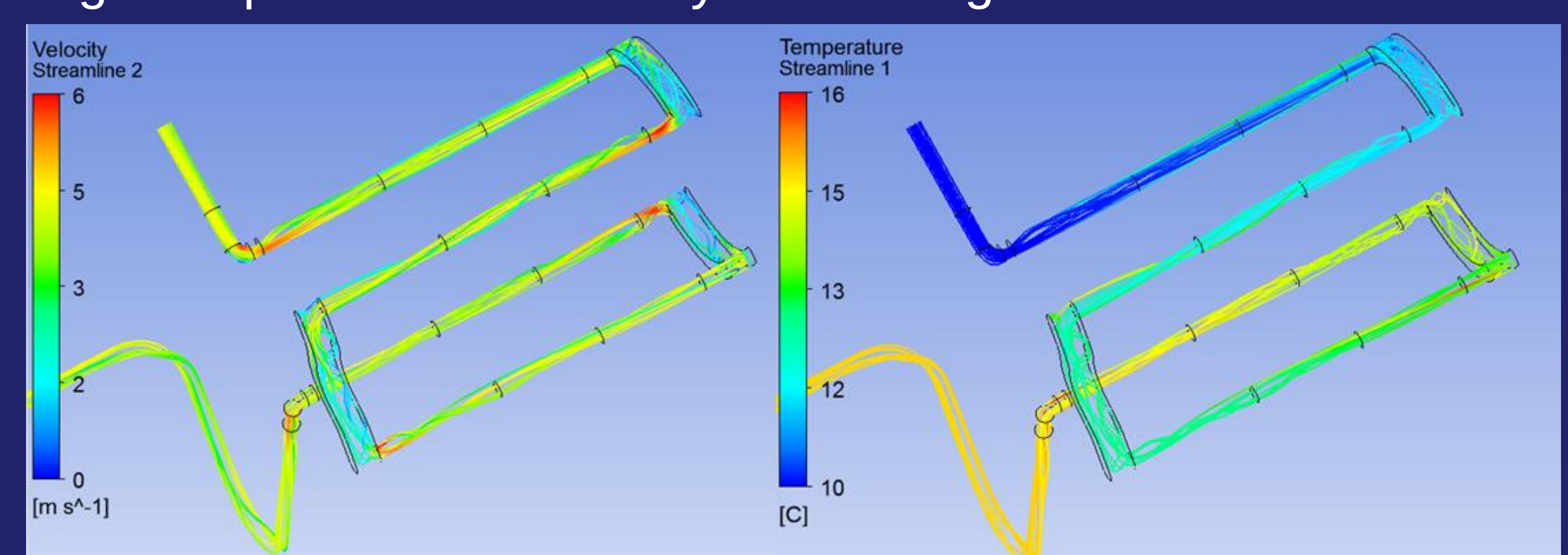
Linac flow streamlines colored as a function of the velocity (left) and the temperature (right)
