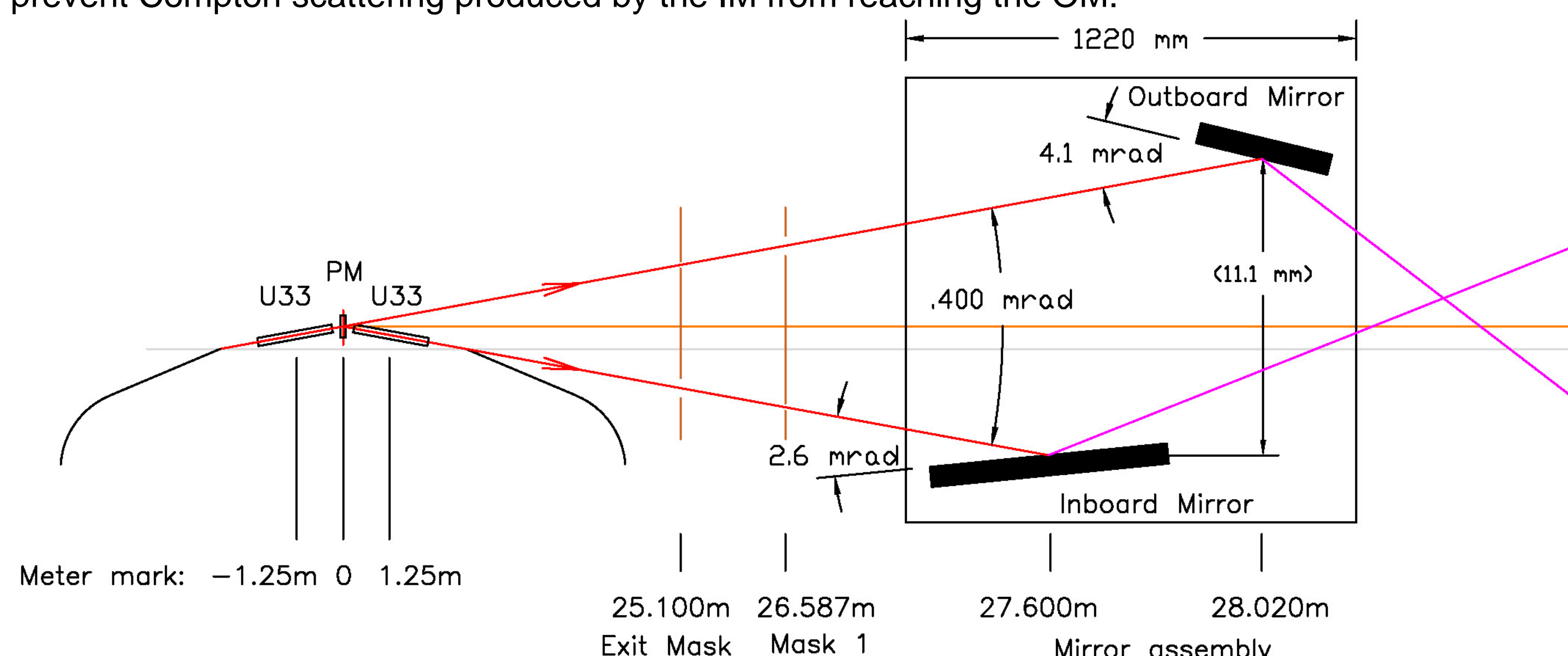
Figure 2. Schematic of the staggered mirror system.
