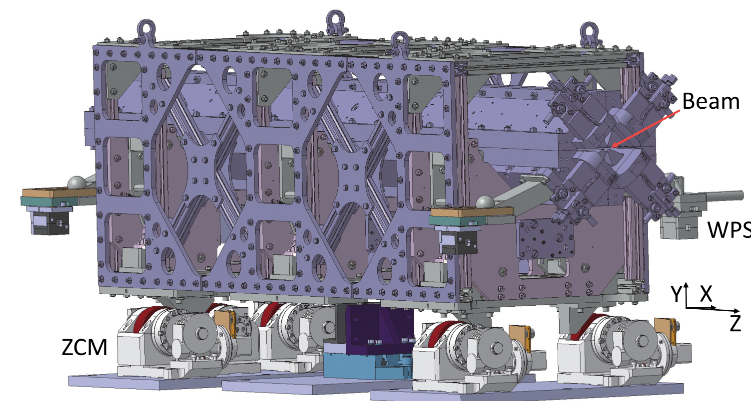
Figure 1. CLIC MBQ and its stabilisation system mounted on cam movers.
