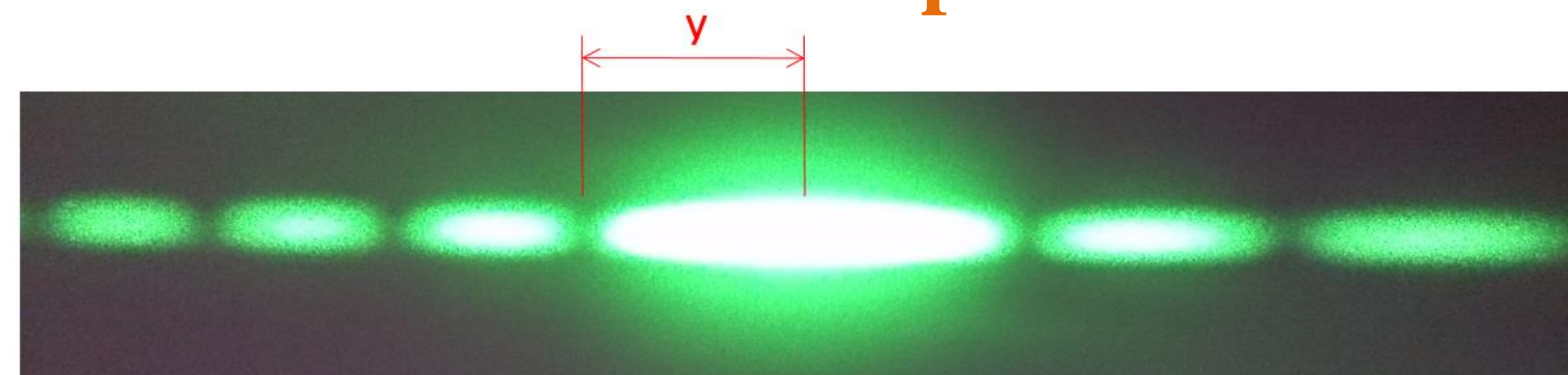
Figure 5: Diffraction pattern observed in the test of parallelism for horizontal slit.
