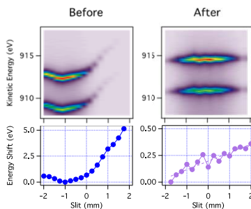
Figure 7: Improved Beamline Performance
