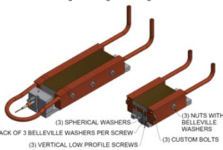
Figure 3: Modified Grating Holder
