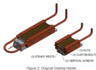
Figure 2: Original Grating Holder
