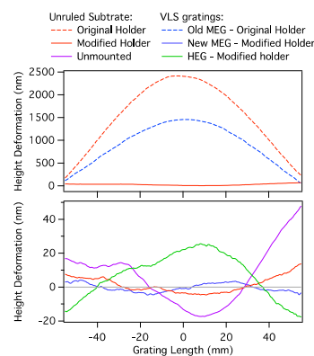
Figure 5: Surface Profile Results
