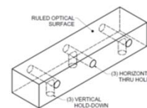
Figure 1: Grating Substrate Mounting Details
