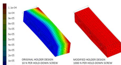
Figure 6: FEA Comparison of Grating Distortions
