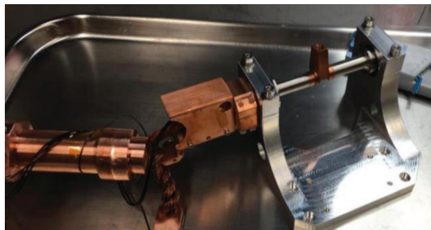
Figure 4: Apparatus used for the preliminary thermal tests. The copper hardware on the left connects to the cryostat (not shown) and an aluminium yoke holds the stainless steel-glidcop sample holder to complete the trunnion assembly.
