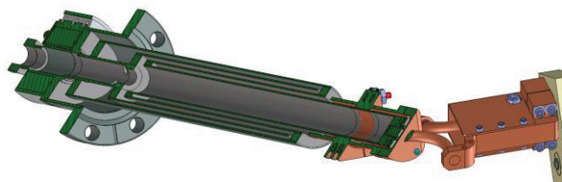
Figure 3: A cross section of the cryostat exhibiting the serpentine design.
