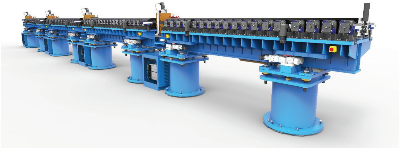
Figure 11: Rendered Image of Hard X-ray Undulator Beamline.
