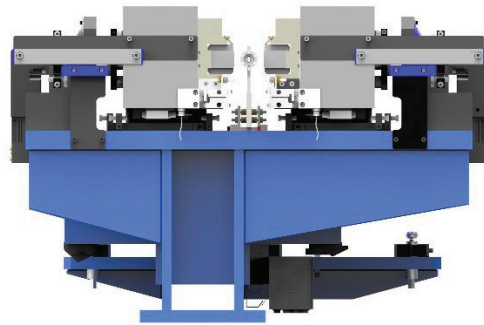
Figure 10: Upstream End View of HGVPU.
