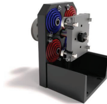
Figure 5: Individual Spring Cage Assembly.
