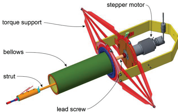
Figure 4: Dedicated feedthrough with strut and piezo.
