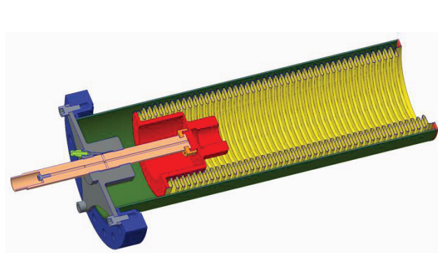
Figure 5: The sliding parts and the UHV-welding assembly.
