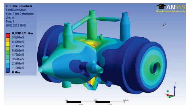
Figure 7: Deformation of the chamber under air pressure.
