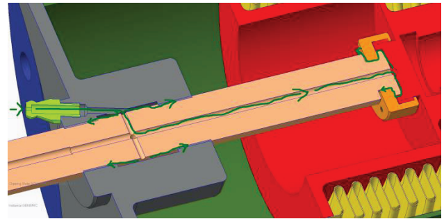
Figure 6: The greasing path for the sliding pairs.
