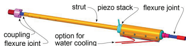
Figure 3: Strut with joints and piezo.
