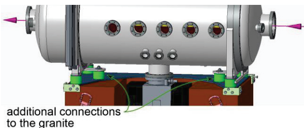
Figure 9: Connection of the chamber to the granite.
