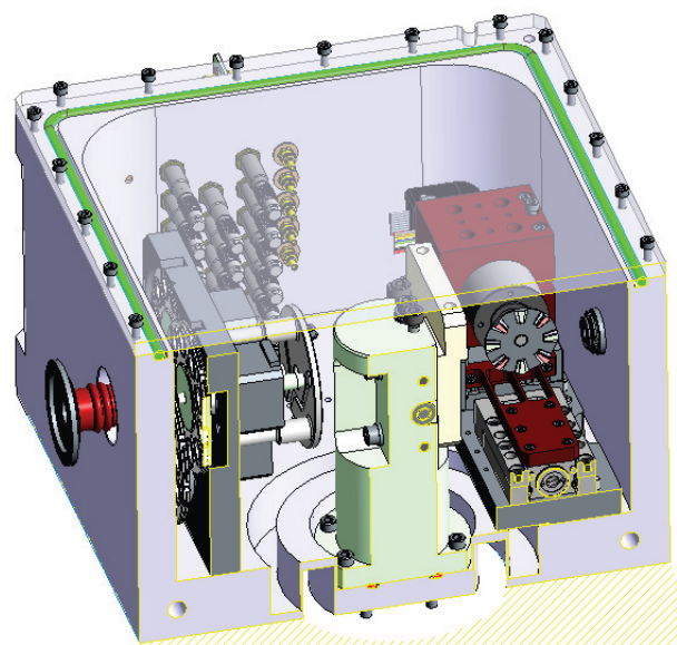
Figure 5: A section view of the beam conditioning assembly.
