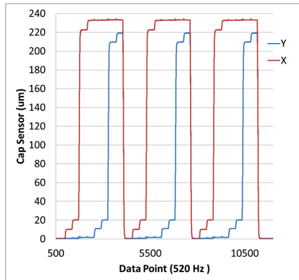
Figure 7: Prototype motion test data set full range,
