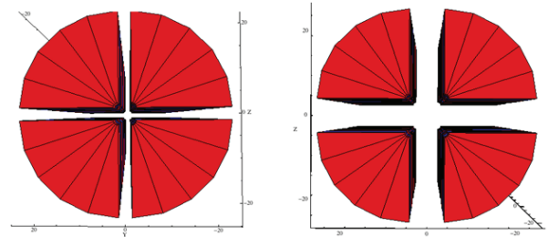
Figure 14: APPLE-X configuration.
