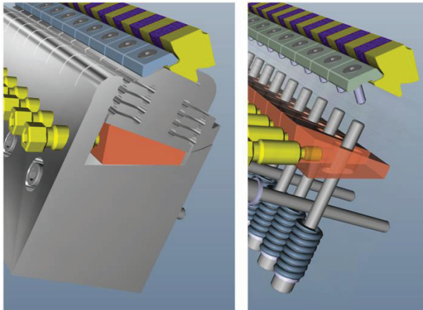
Figure 17: Keeper design.
