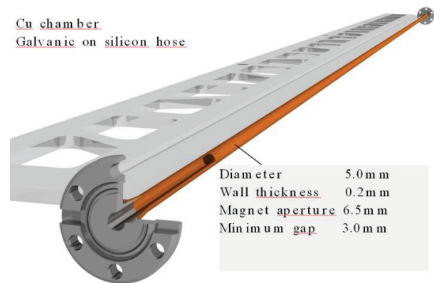
Figure 18: Vacuum Chamber.
