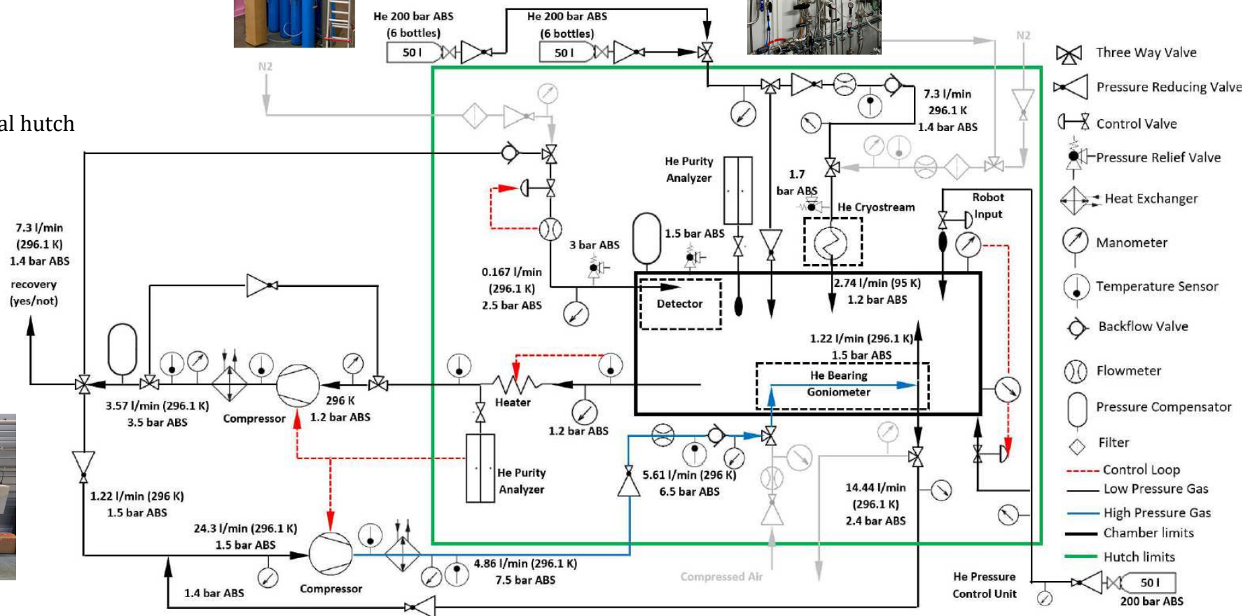
Circuit manifold panel In Experimental hutch
