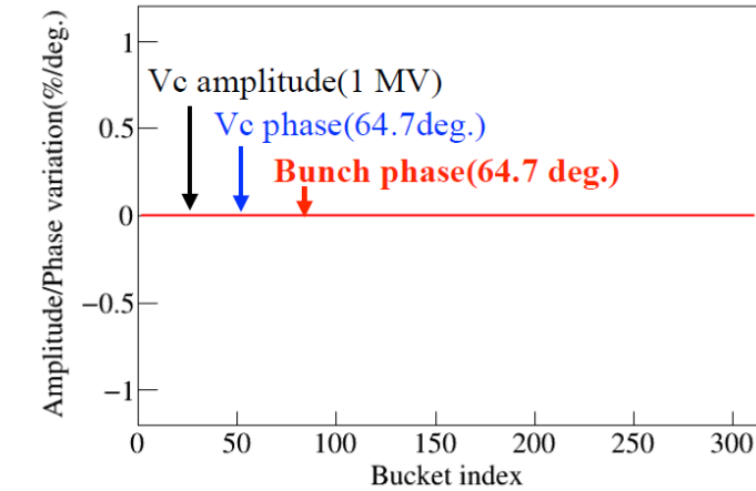
Fig.1 Cavity voltage and bunch phase with uniform filling
