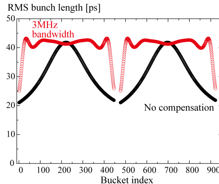
c) Bunch length along the train w/wo. Compensation signal
